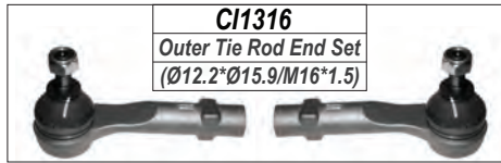
CI1416 Rack End (14*1.5/16*1.5/312)
