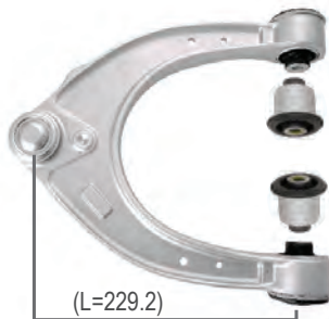
BM1728 Upper Control Arm
